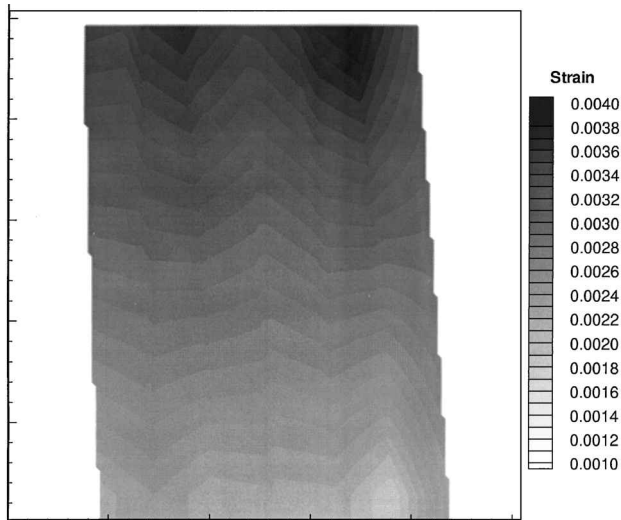
Fig. 9 Two-dimensional thermally induced strain field resulting from an imposed one-dimensional temperature distribution.
