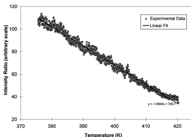
Fig. 6 Normalized phosphor intensity distribution vs temperature.
