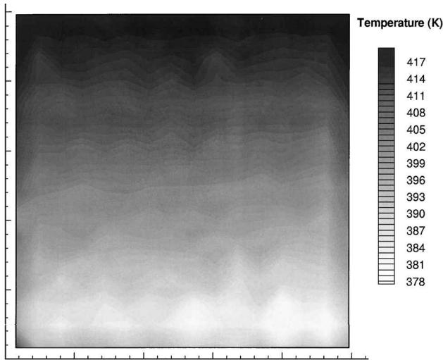
Fig. 7 Temperature distribution in central 1.27 \times 0.5 cm section of test sample.
