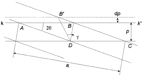
Fig. 2 Geometric relationship between a reference and a strained line array.
