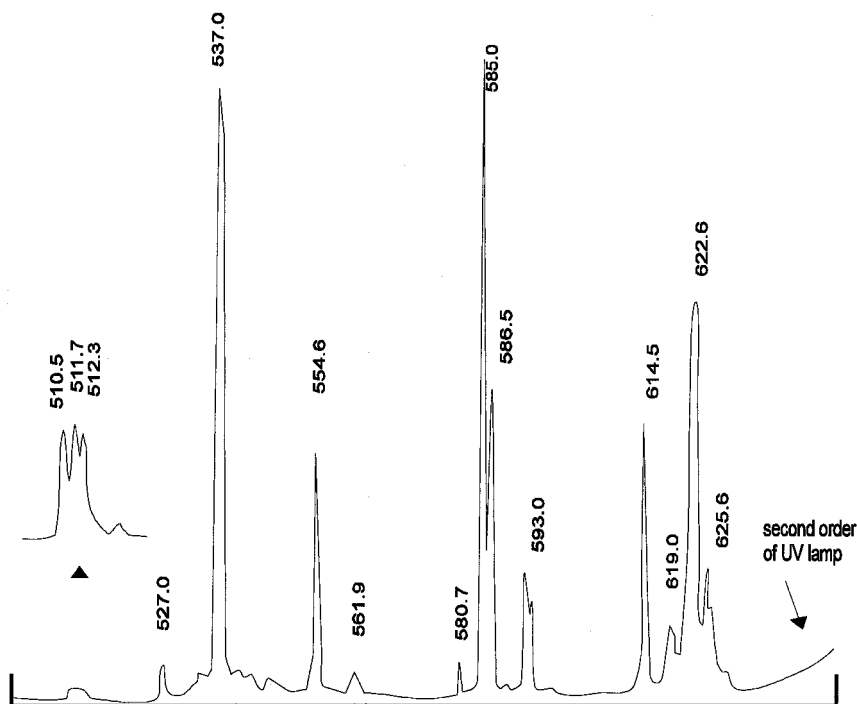
Fig. 3 Emission spectrum of \text{La}_2\text{O}_2\text{S:Eu}^{+3} excited by broadband uv at room temperature.
