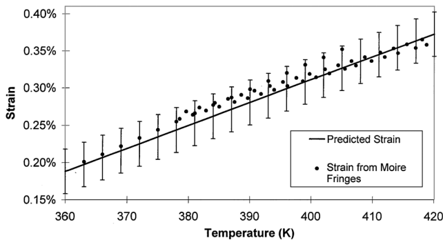
Fig. 8 Comparison of imaged normal strain measurement with coefficient of thermal expansion prediction.
