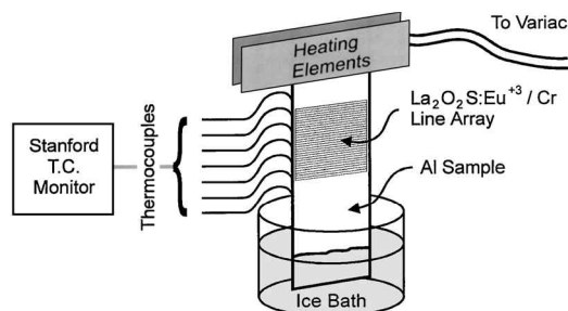
Fig. 5 Schematic of one-dimensional temperature and thermal strain field apparatus.
