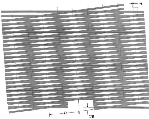
Fig. 1 Moiré fringes formed from two unstrained arrays.
